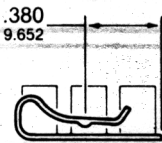
TO-127 CASE 7-291
